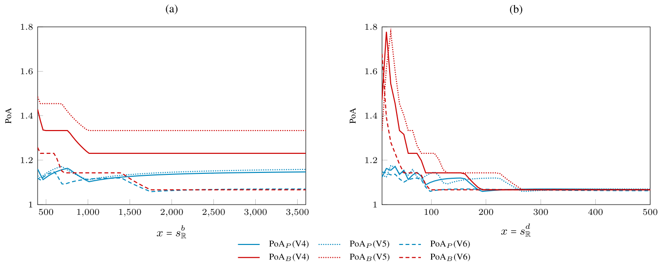
FIGURE 5. Price of anarchy ( \Theta_P : \Theta_{Opt} ) following changes in platform parameters. (a) Increase in remote processing speed. (b) Increase in wireless bandwidth.
