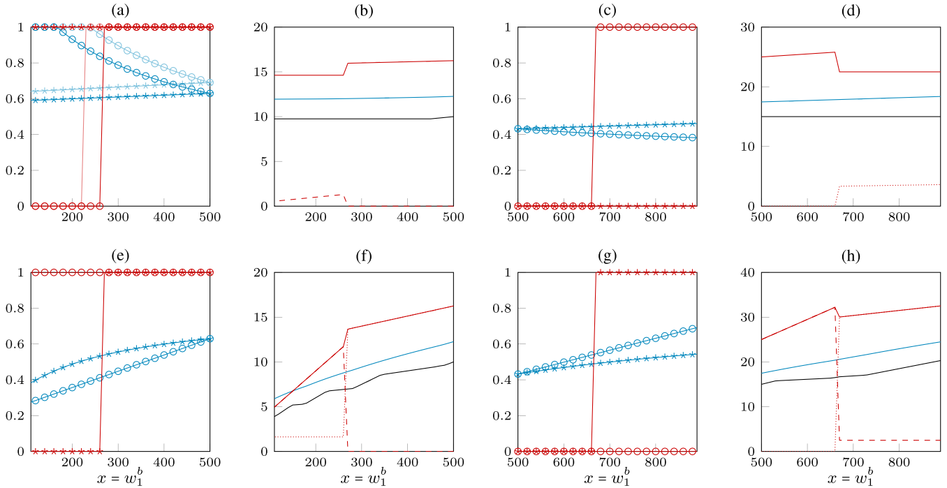
FIGURE 3. Offload Strategy Behaviour. Non-Cooperative incomplete information: a_1^{\mathbb{R}} \circ , a_i^{\mathbb{R}} \times , \Theta_B^{\mathbb{N}} \cdots , \Theta_B^{\mathbb{R}} \text{---} , \Theta_B^{\mathbb{R}} \text{-- --} ; non-cooperative complete information (Nash): p_1^{\mathbb{R}} \circ , p_i^{\mathbb{R}} \times , \Theta_p \text{---} and Cooperative Offload: \Theta_{Opt} \text{---} . (a) Strategies (S1&S1F). (b) Social costs (S1). (c) Strategies (S2). (d) Social costs (S2). (e) Strategies (S3). (f) Social costs (S3). (g) Strategies (S4). (h) Social costs (S4).
